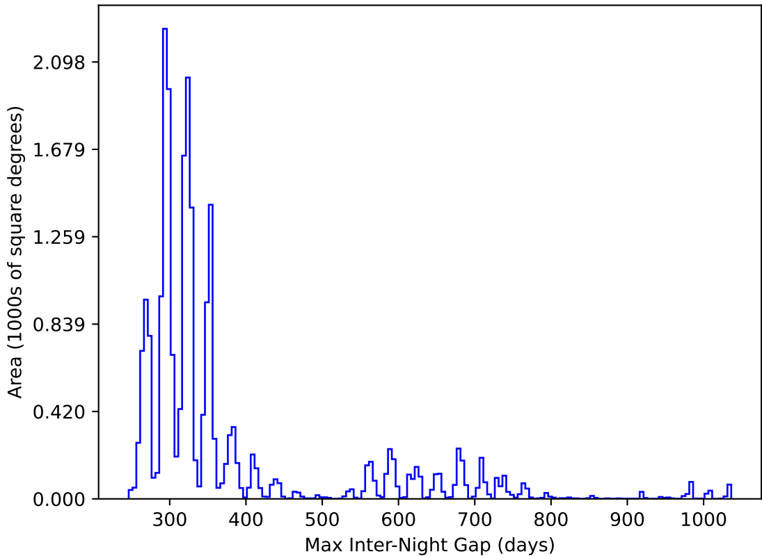
too_elab_r128_d3_gz_v3.4_10yrs All sky y band: Max Inter-Night Gap
