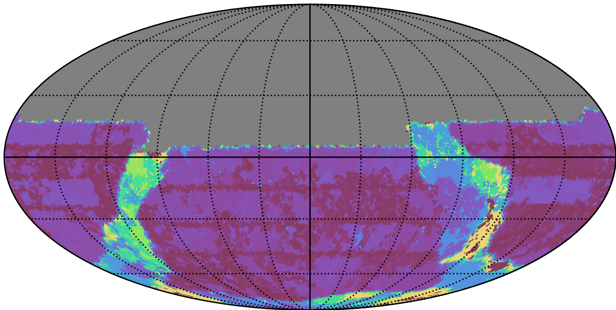
too_elab_r128_d3_gz_v3.4_10yrs All sky u band: Max Inter-Night Gap
