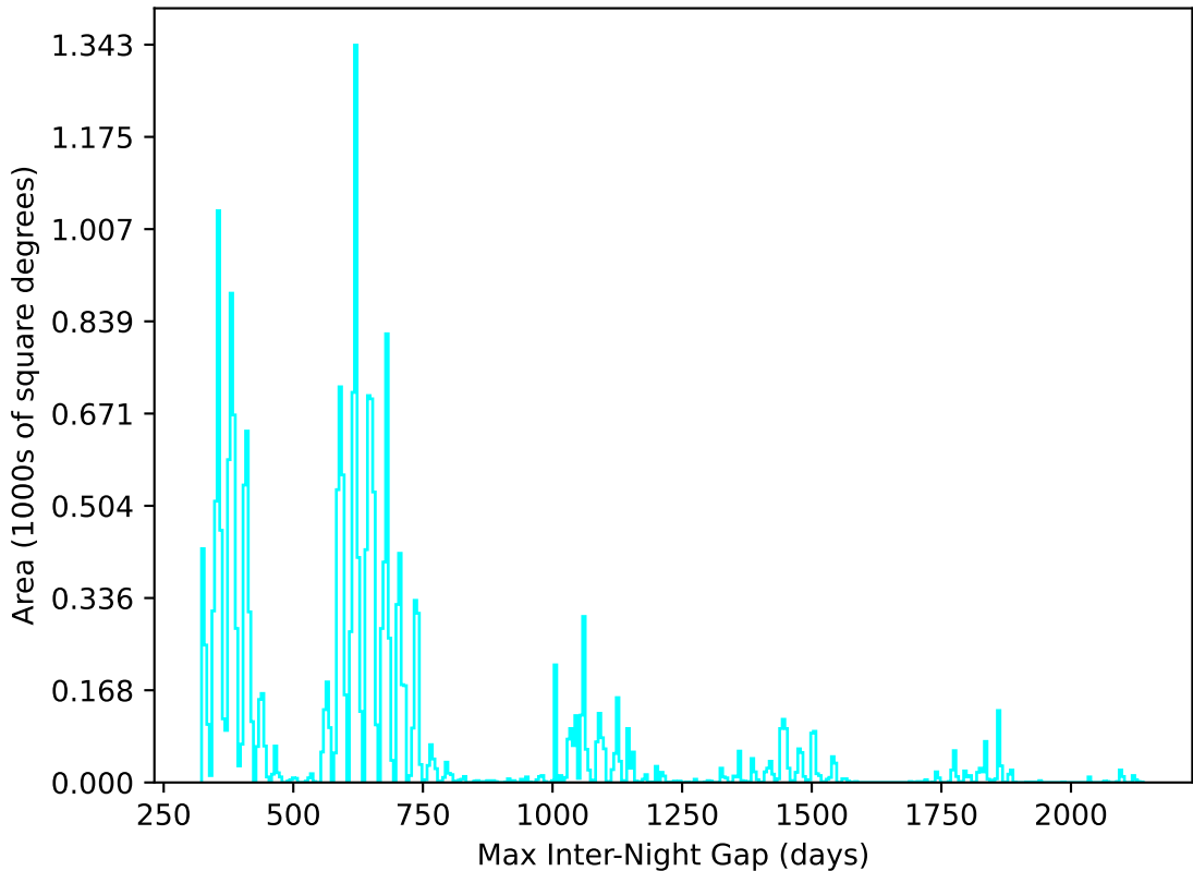
too_elab_r128_d3_gz_v3.4_10yrs All sky u band: Max Inter-Night Gap
