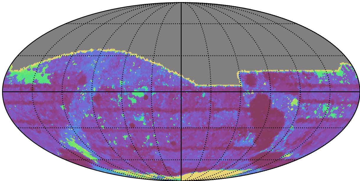
too_elab_r128_d3_gz_v3.4_10yrs All sky r band: Max Inter-Night Gap
