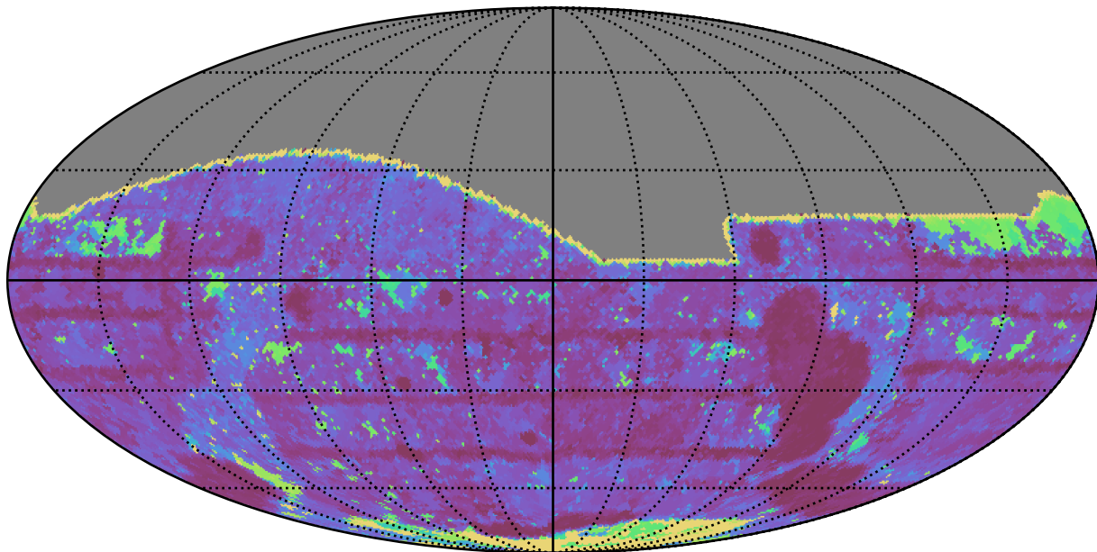
too_elab_r128_d3_gz_v3.4_10yrs All sky i band: Max Inter-Night Gap
