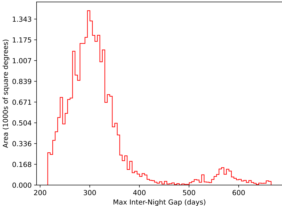
too_elab_r128_d3_gz_v3.4_10yrs All sky i band: Max Inter-Night Gap
