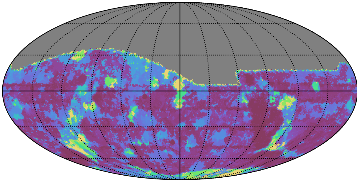
too_elab_r128_d3_gz_v3.4_10yrs All sky g band: Max Inter-Night Gap
