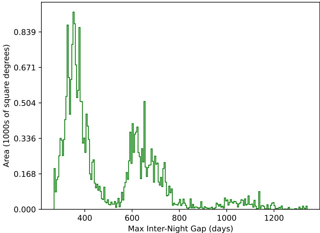
too_elab_r128_d3_gz_v3.4_10yrs All sky g band: Max Inter-Night Gap
