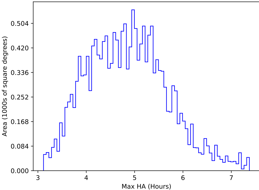
too_elab_r128_d3_gz_v3.4_10yrs WFD z band: Max HA
