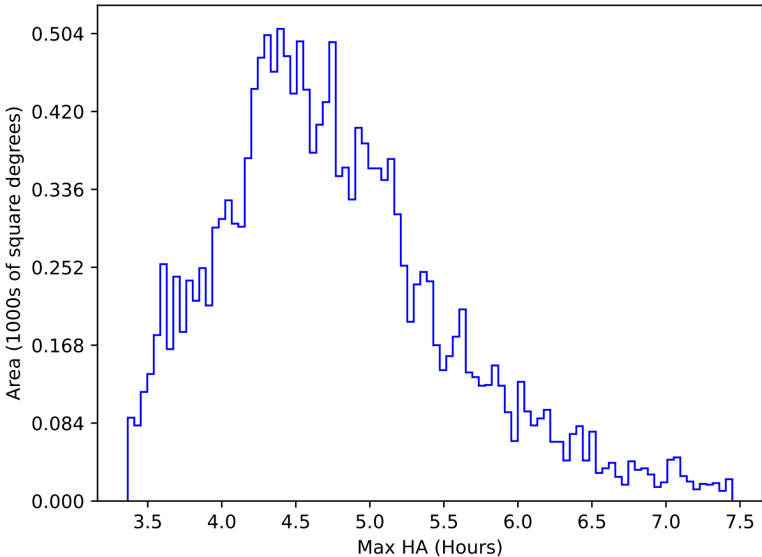
too_elab_r128_d3_gz_v3.4_10yrs WFD y band: Max HA
