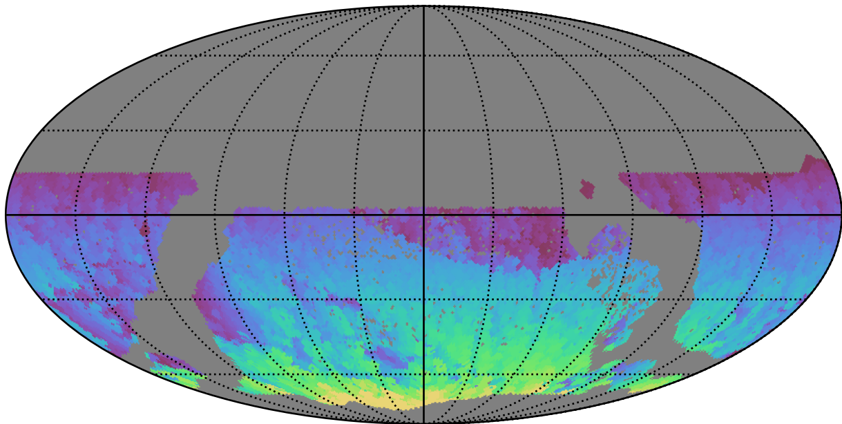
too_elab_r128_d3_gz_v3.4_10yrs WFD i band: Max HA
