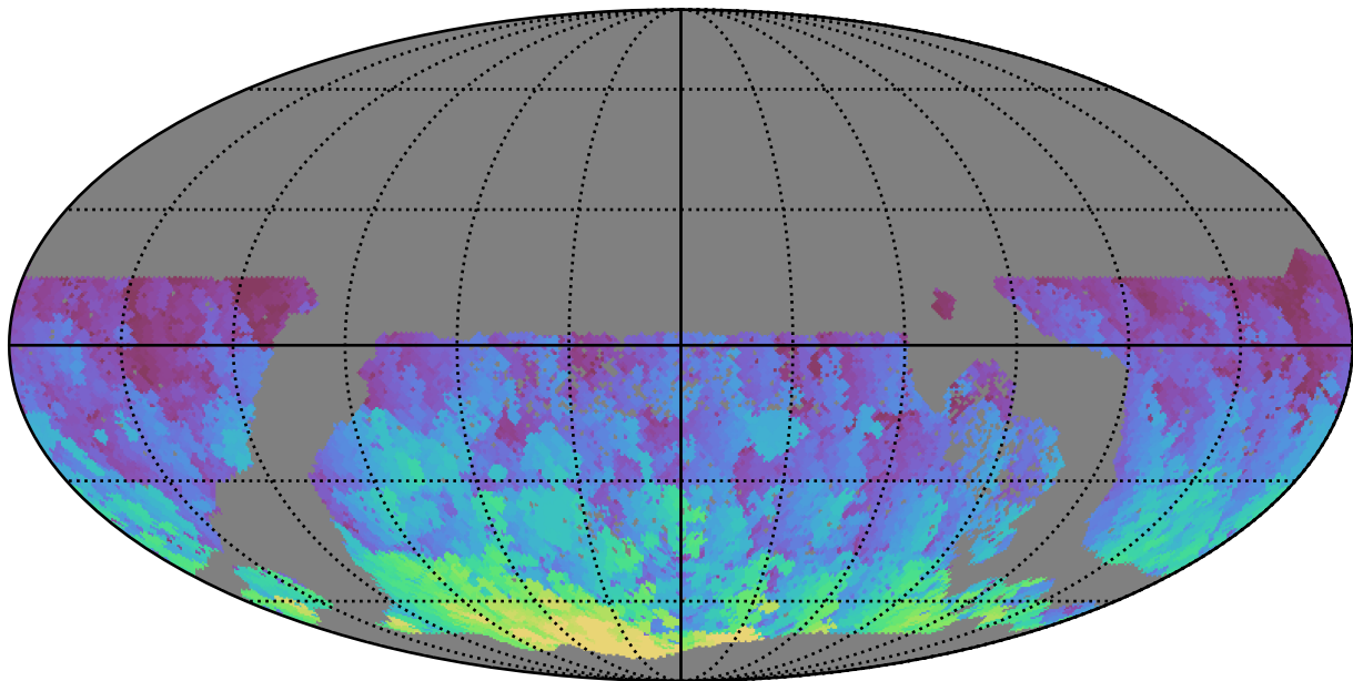
too_elab_r128_d3_gz_v3.4_10yrs WFD g band: Max HA
