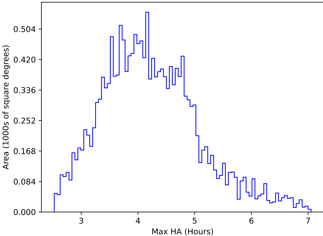
too_elab_r128_d3_gz_v3.4_10yrs WFD g band: Max HA
