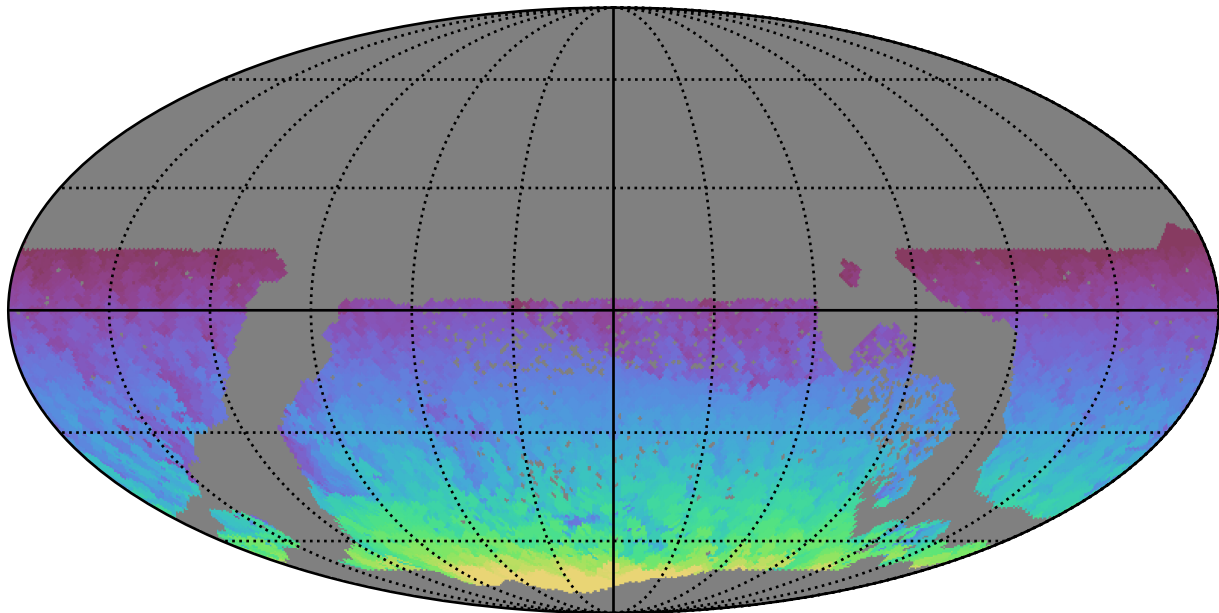
too_elab_r128_d3_gz_v3.4_10yrs WFD all bands: Max HA
