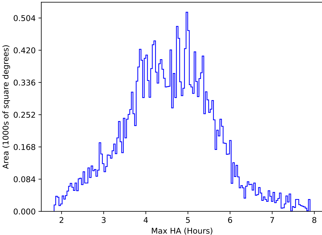
too_elab_r128_d3_gz_v3.4_10yrs All sky z band: Max HA
