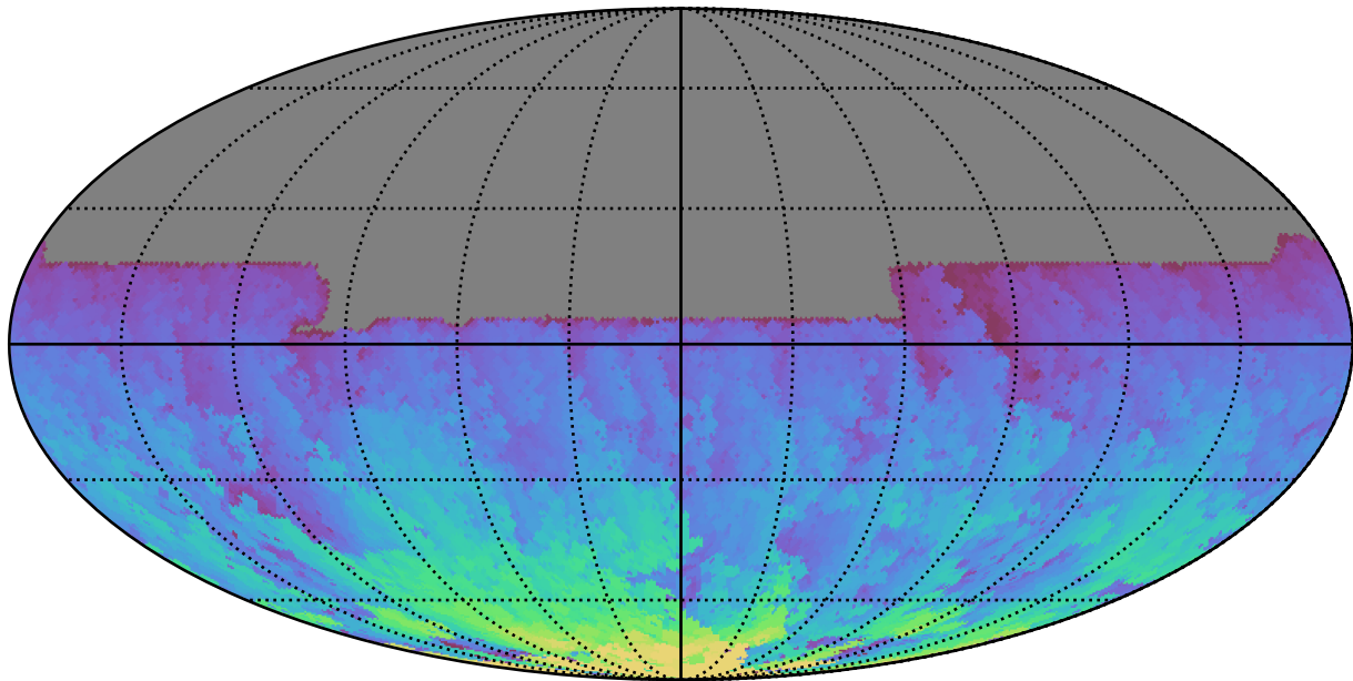
too_elab_r128_d3_gz_v3.4_10yrs All sky y band: Max HA
