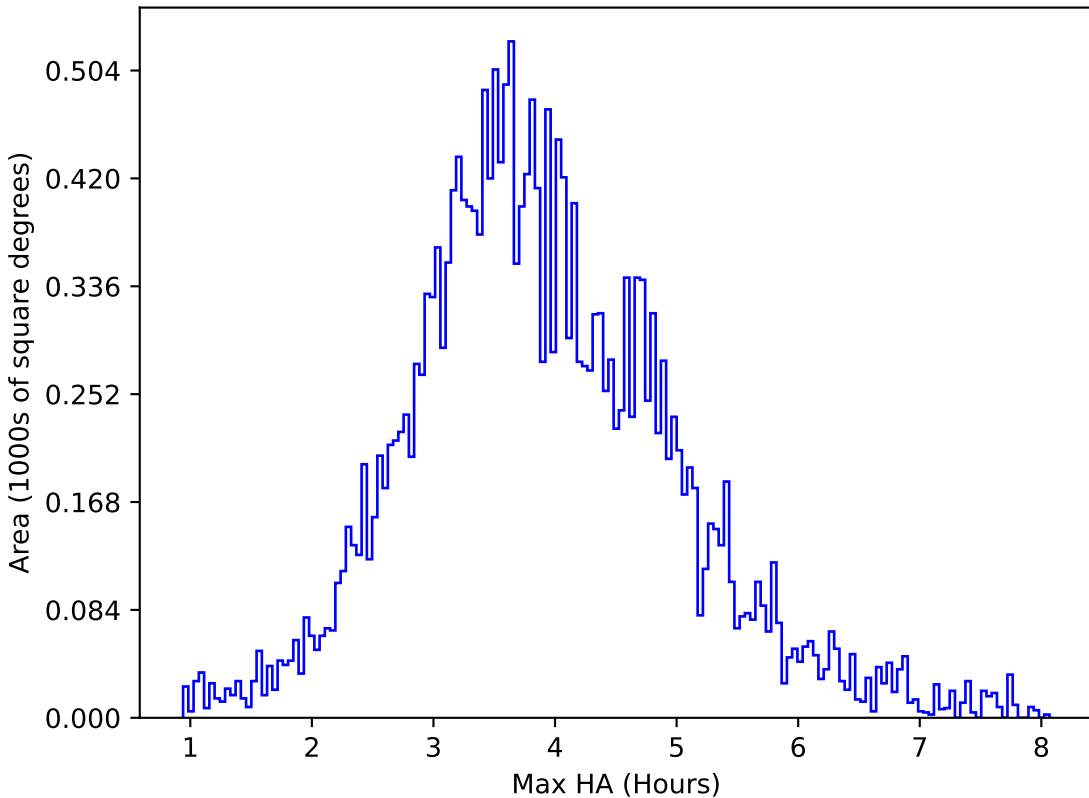
too_elab_r128_d3_gz_v3.4_10yrs All sky u band: Max HA
