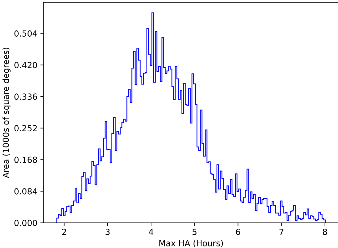
too_elab_r128_d3_gz_v3.4_10yrs All sky r band: Max HA
