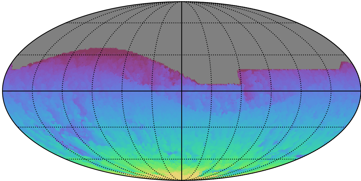
too_elab_r128_d3_gz_v3.4_10yrs All sky all bands: Max HA
