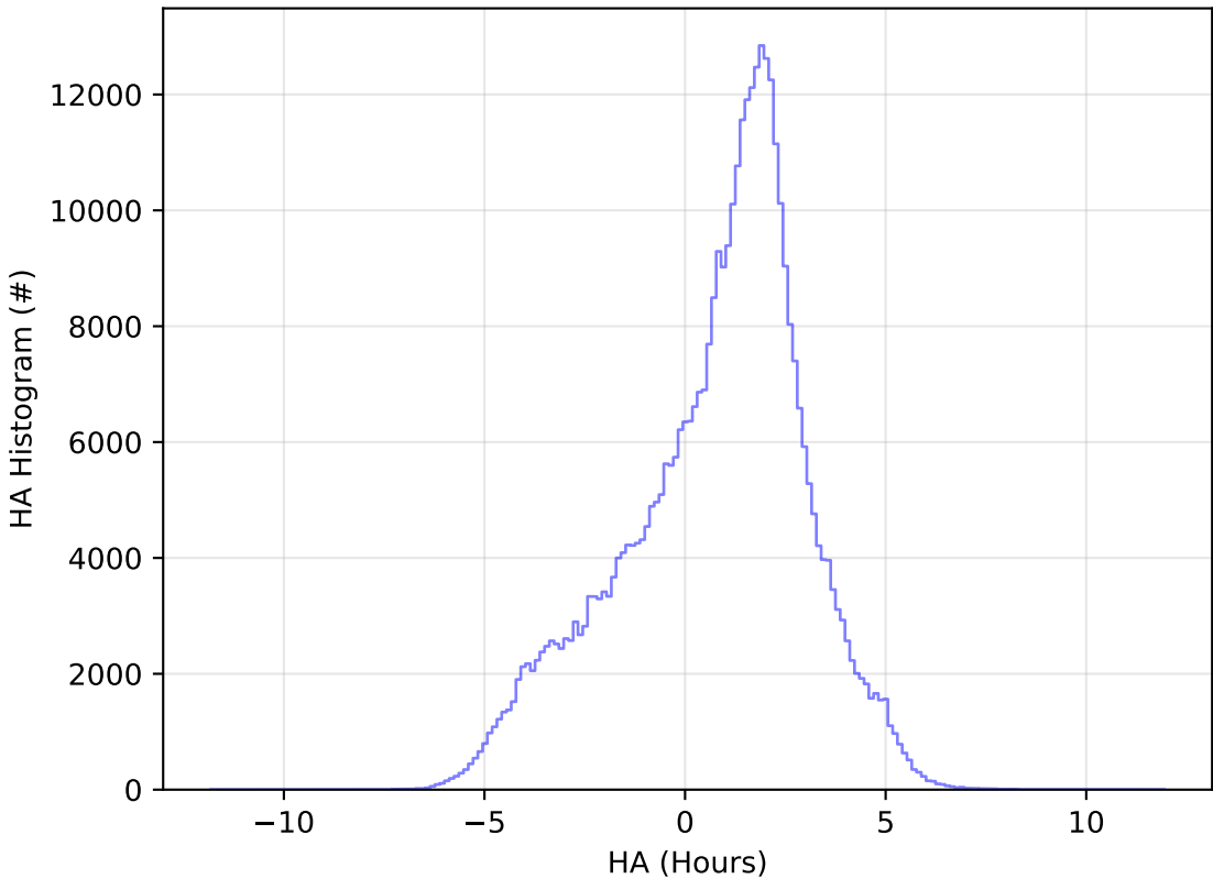
too_elab_r128_d3_gz_v3.4_10yrs WFD z band: HA Histogram
