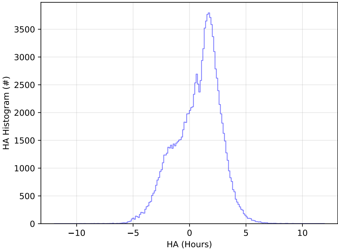
too_elab_r128_d3_gz_v3.4_10yrs WFD u band: HA Histogram
