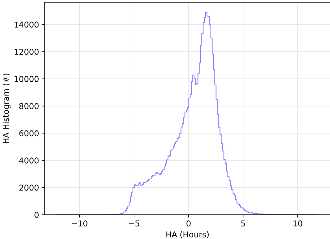
too_elab_r128_d3_gz_v3.4_10yrs WFD r band: HA Histogram
