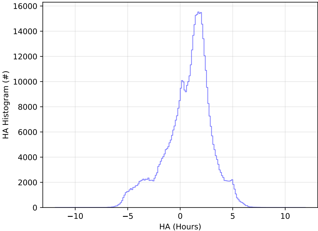
too_elab_r128_d3_gz_v3.4_10yrs WFD i band: HA Histogram
