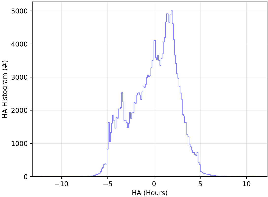
too_elab_r128_d3_gz_v3.4_10yrs WFD g band: HA Histogram
