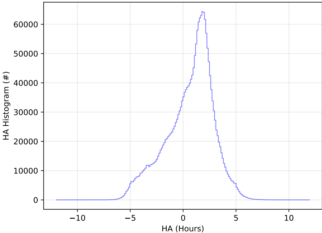
too_elab_r128_d3_gz_v3.4_10yrs WFD all bands: HA Histogram
