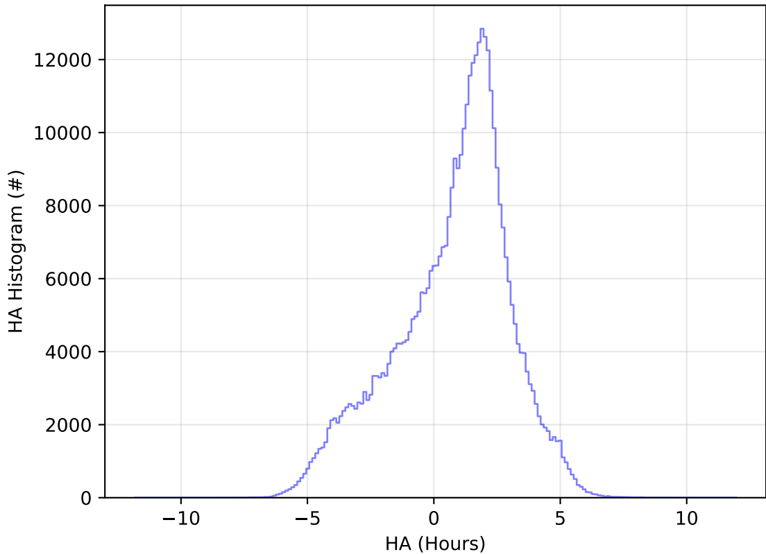
too_elab_r128_d3_gz_v3.4_10yrs All sky z band: HA Histogram
