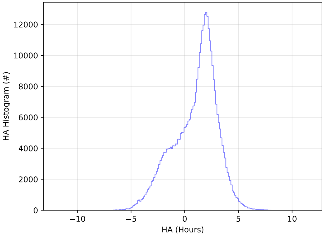
too_elab_r128_d3_gz_v3.4_10yrs All sky y band: HA Histogram
