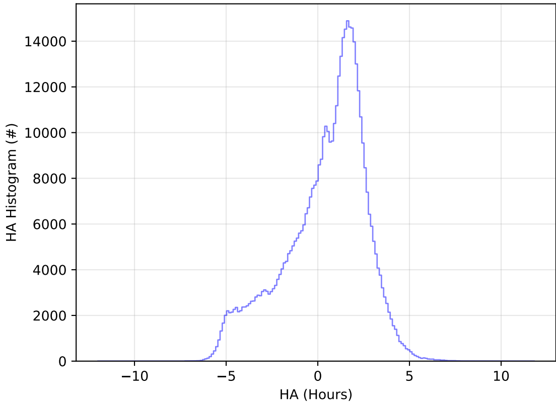
too_elab_r128_d3_gz_v3.4_10yrs All sky r band: HA Histogram
