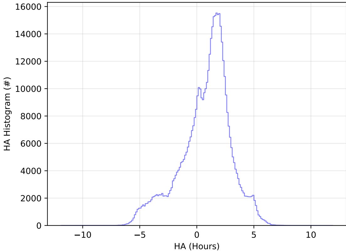
too_elab_r128_d3_gz_v3.4_10yrs All sky i band: HA Histogram
