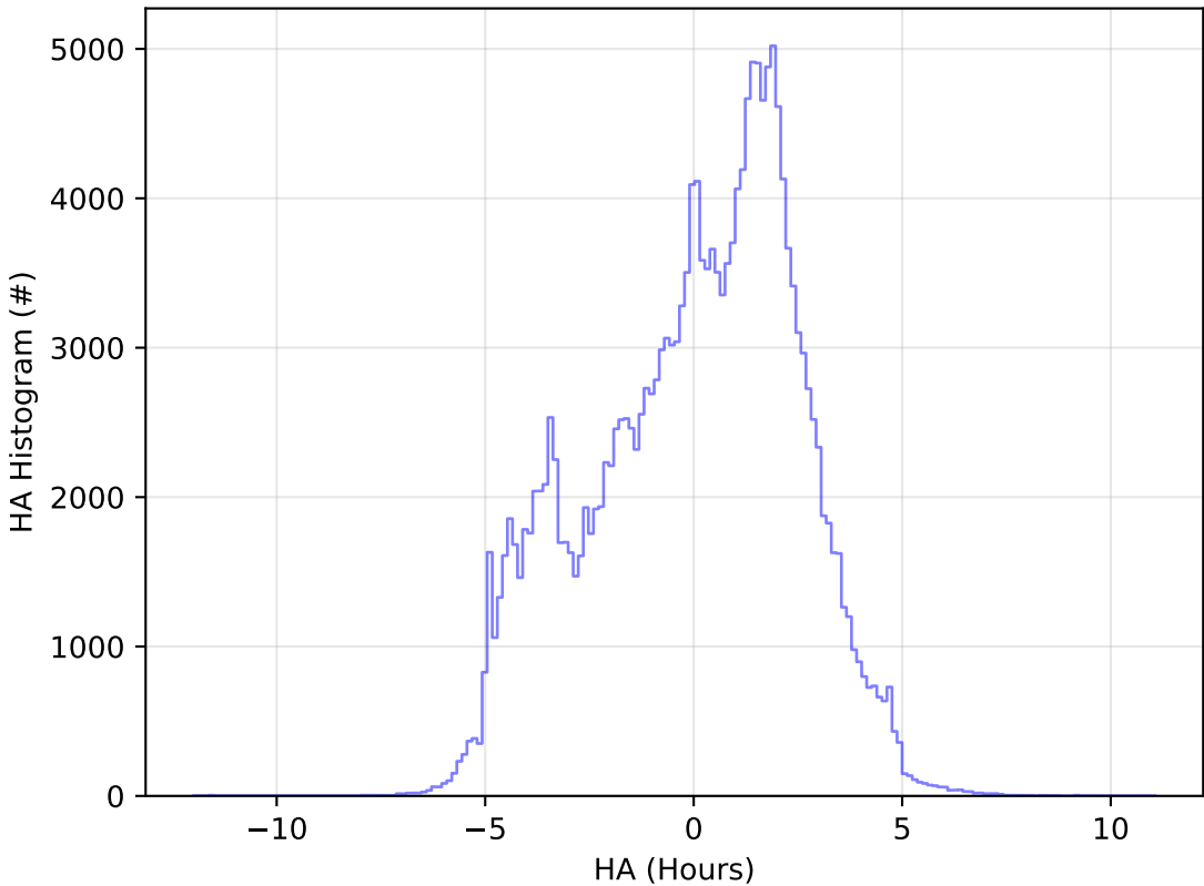
too_elab_r128_d3_gz_v3.4_10yrs All sky g band: HA Histogram
