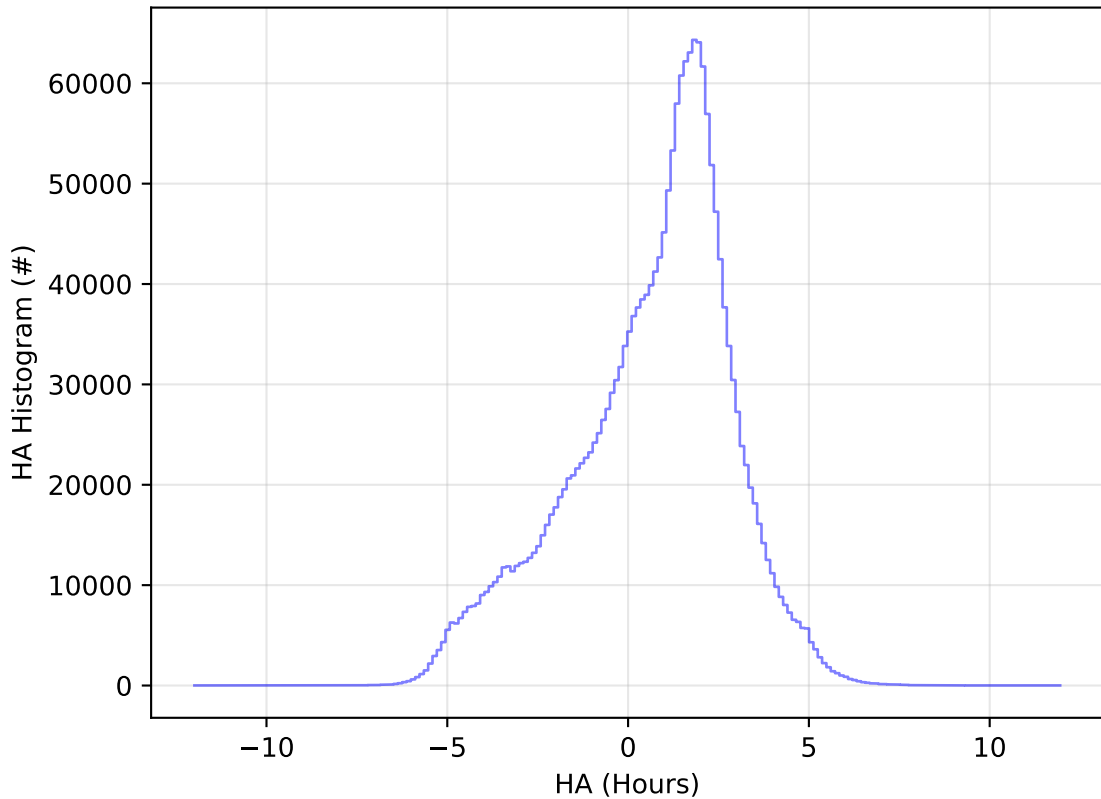
too_elab_r128_d3_gz_v3.4_10yrs All sky all bands: HA Histogram
