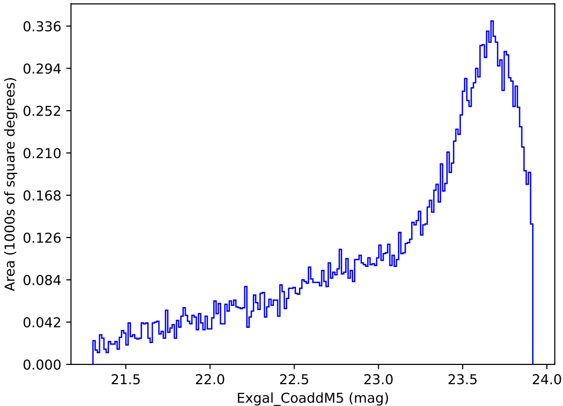
too_elab_r128_d3_gz_v3.4_10yrs Yr 3-4 y band: Exgal_CoaddM5
