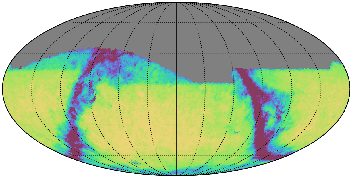
too_elab_r128_d3_gz_v3.4_10yrs Yr 1 r band: Exgal_CoaddM5
