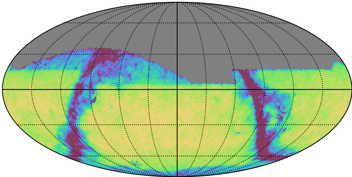
too_elab_r128_d3_gz_v3.4_10yrs Yr 1 i band: Exgal_CoaddM5
