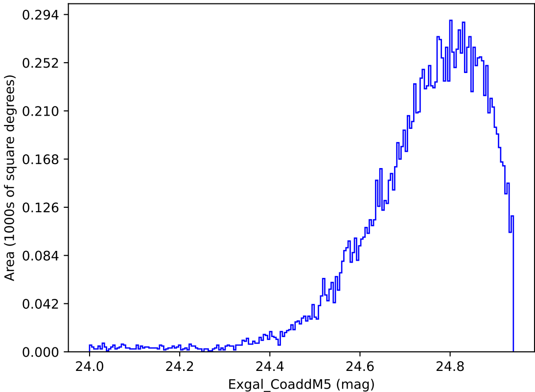
too_elab_r128_d3_gz_v3.4_10yrs WFD y band: Exgal_CoaddM5
