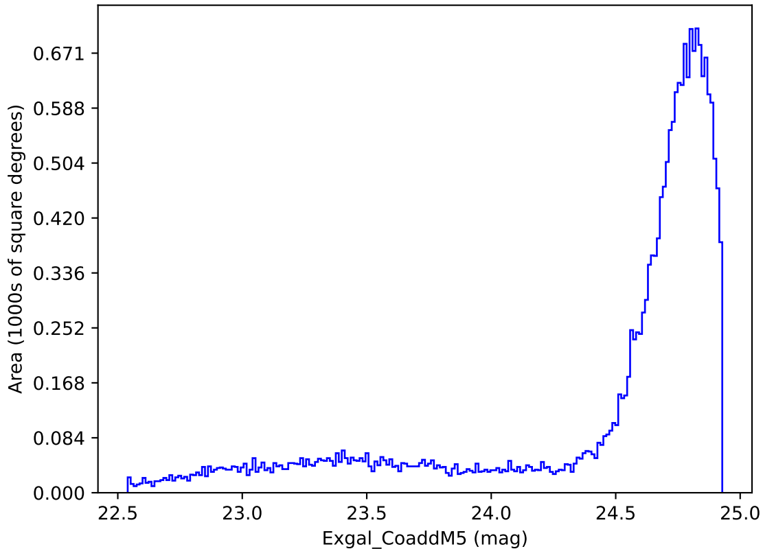
too_elab_r128_d3_gz_v3.4_10yrs All sky y band: Exgal_CoaddM5
