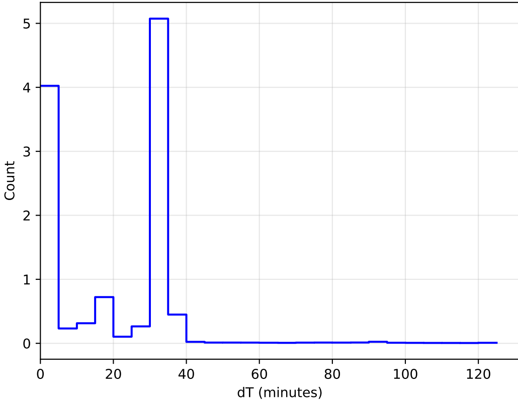
too_elab_r128_d3_gz_v3.4_10yrs WFD: DeltaT Histogram 1e6
