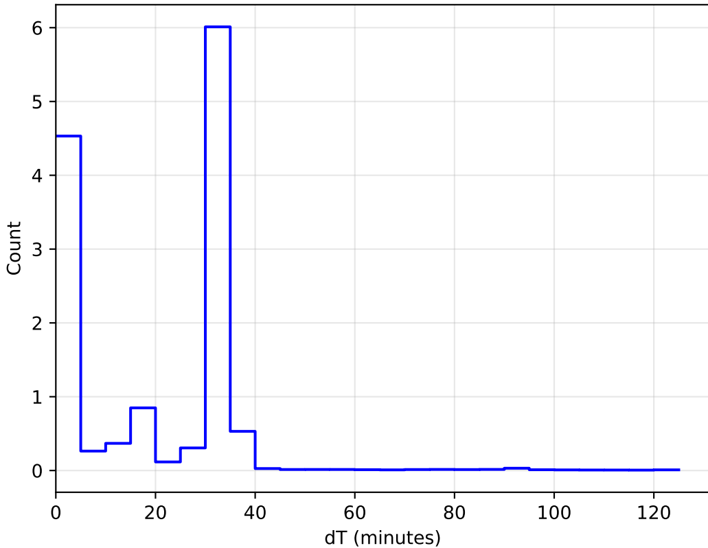
too_elab_r128_d3_gz_v3.4_10yrs All sky: DeltaT Histogram 1e6
