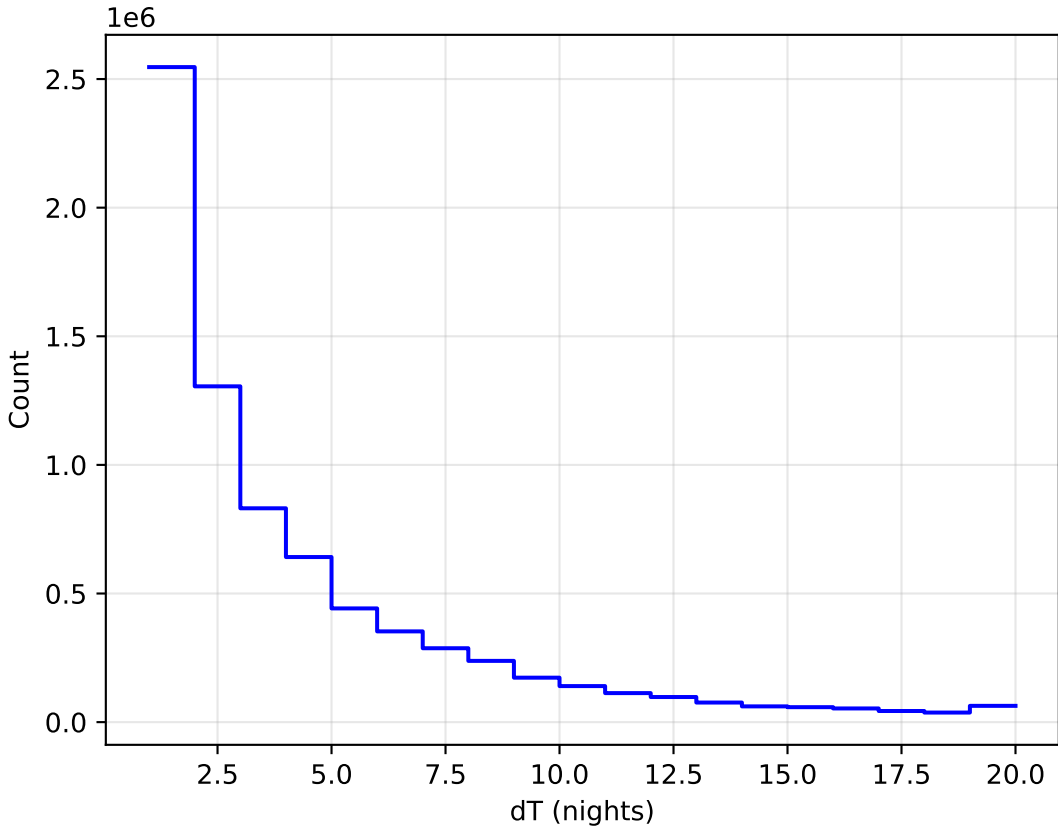
too_elab_r128_d3_gz_v3.4_10yrs WFD all bands: DeltaNight Histogram
