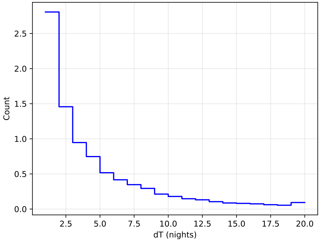
too_elab_r128_d3_gz_v3.4_10yrs All sky all bands: DeltaNight Histogram
