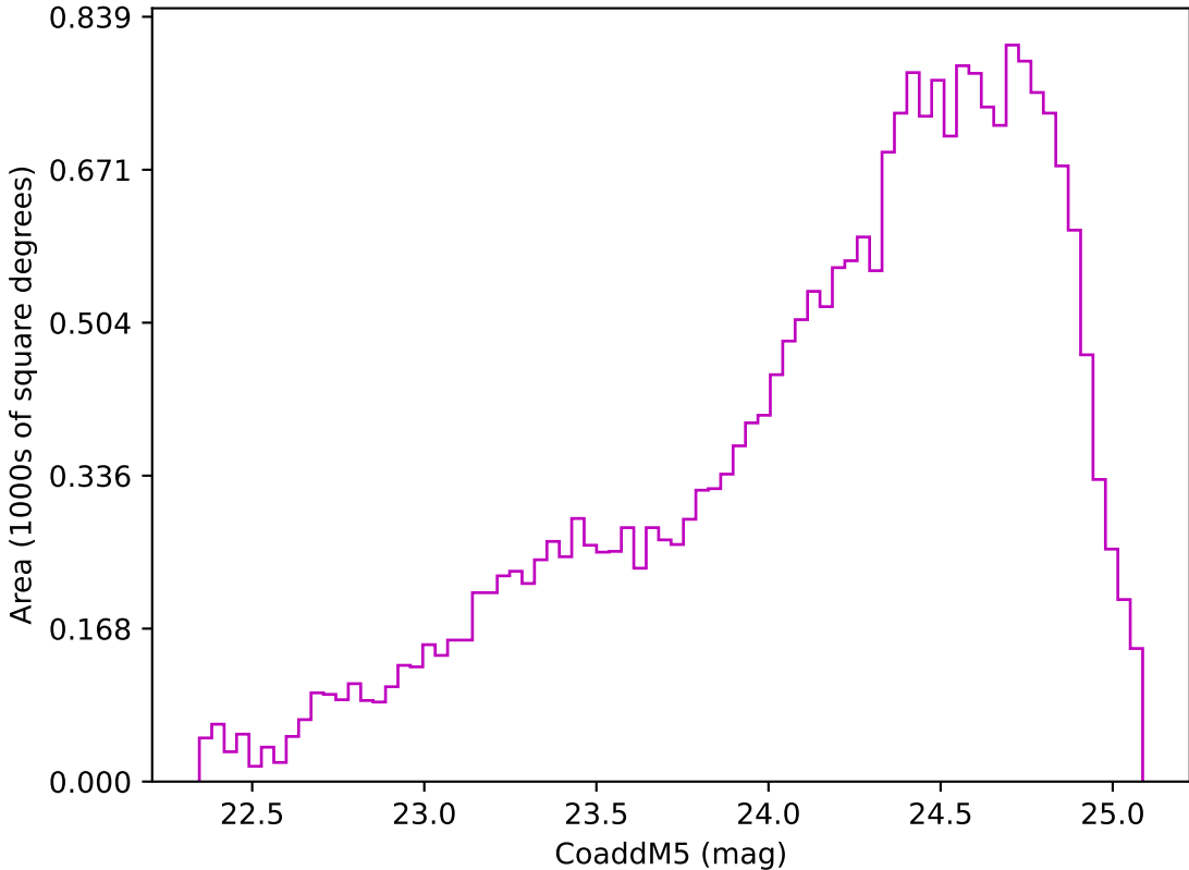
too_elab_r128_d3_gz_v3.4_10yrs Yr 3-4 z band: CoaddM5
