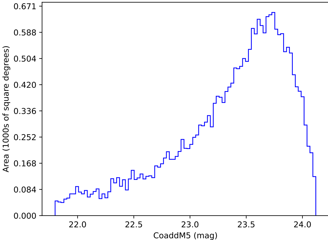
too_elab_r128_d3_gz_v3.4_10yrs Yr 3-4 y band: CoaddM5
