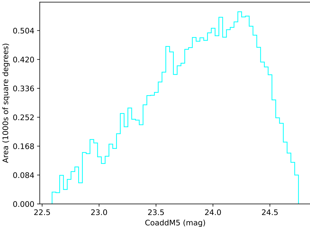
too_elab_r128_d3_gz_v3.4_10yrs Yr 3-4 u band: CoaddM5
