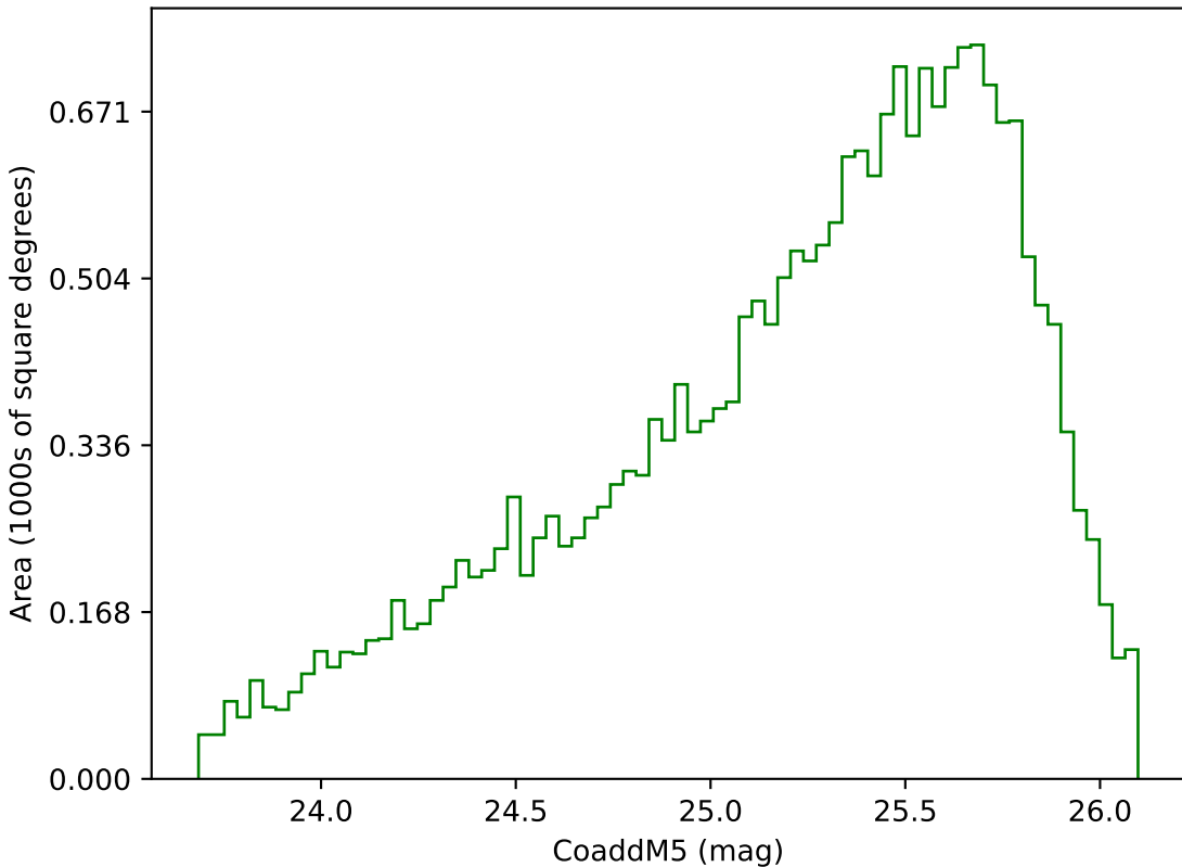
too_elab_r128_d3_gz_v3.4_10yrs Yr 3-4 g band: CoaddM5
