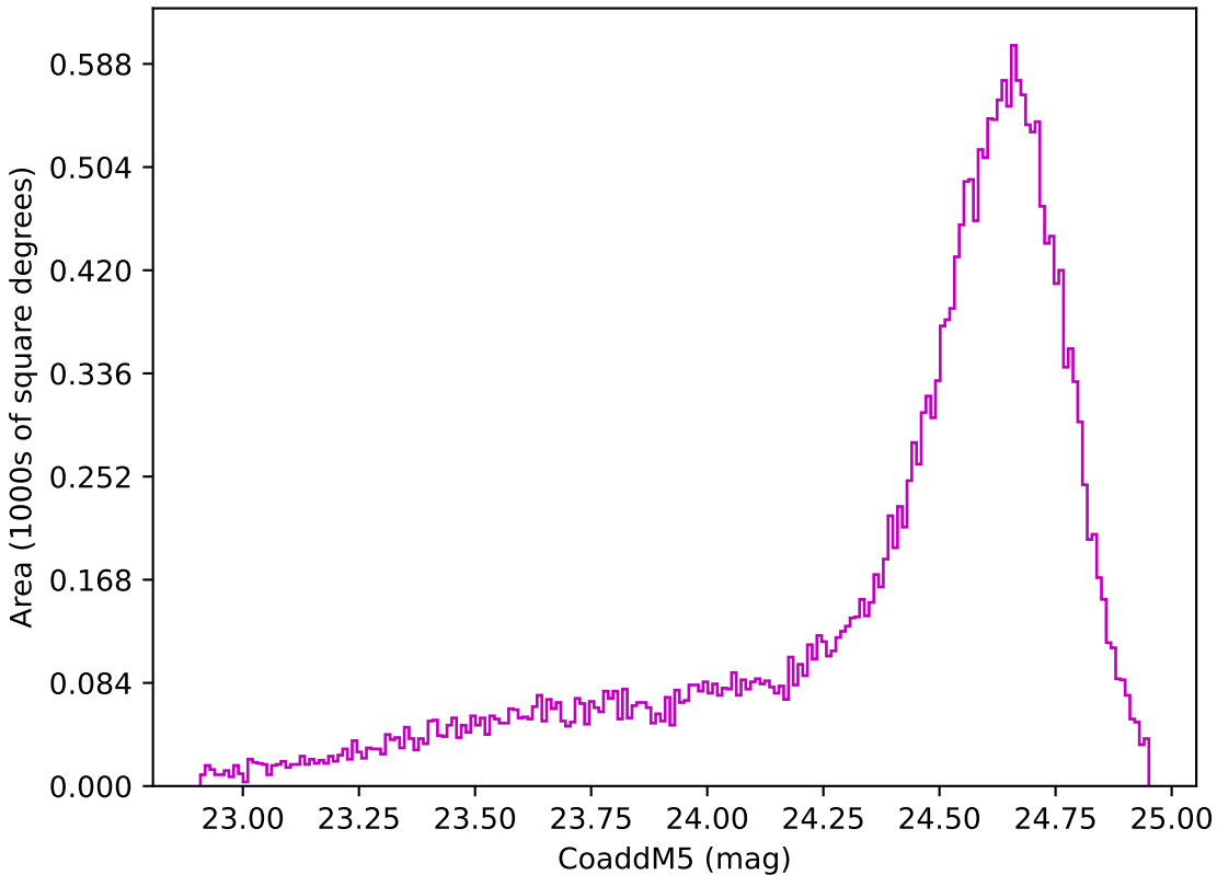
too_elab_r128_d3_gz_v3.4_10yrs Yr 1 z band: CoaddM5
