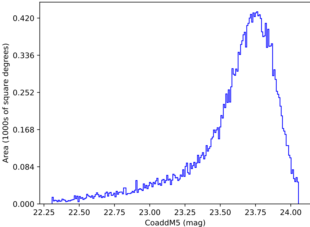
too_elab_r128_d3_gz_v3.4_10yrs Yr 1 y band: CoaddM5
