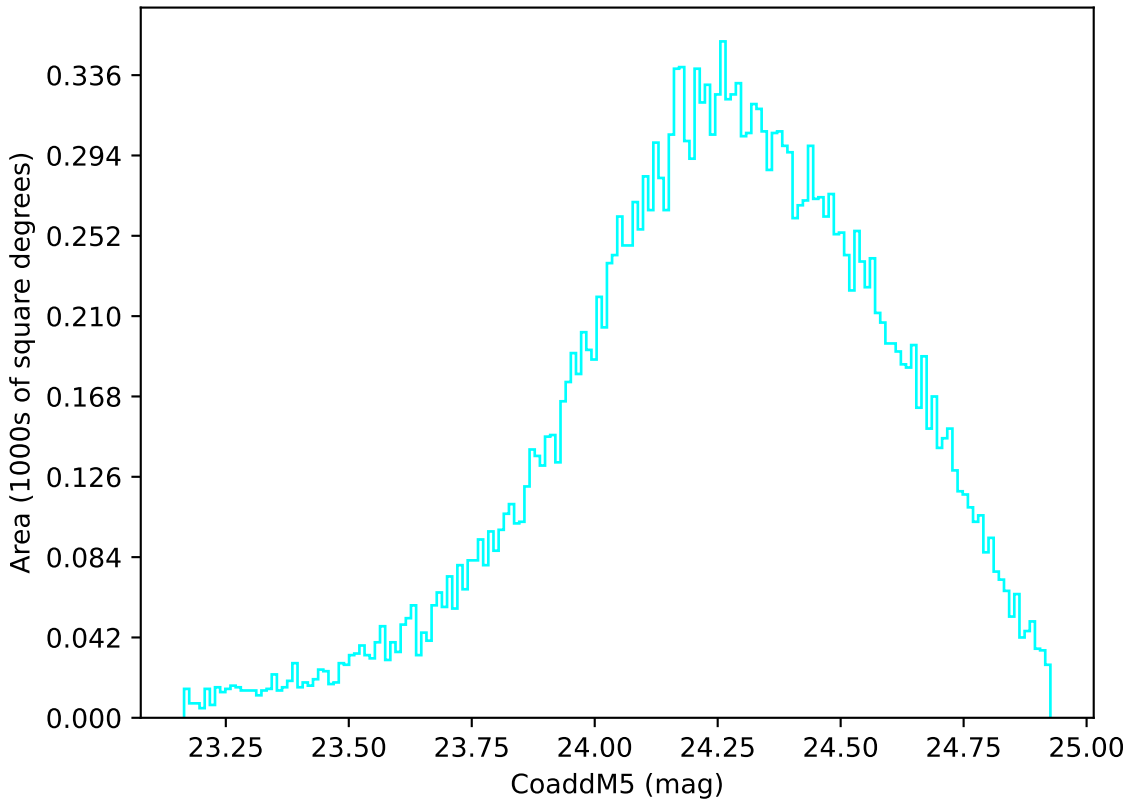
too_elab_r128_d3_gz_v3.4_10yrs Yr 1 u band: CoaddM5
