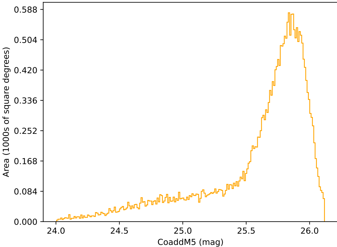
too_elab_r128_d3_gz_v3.4_10yrs Yr 1 r band: CoaddM5
