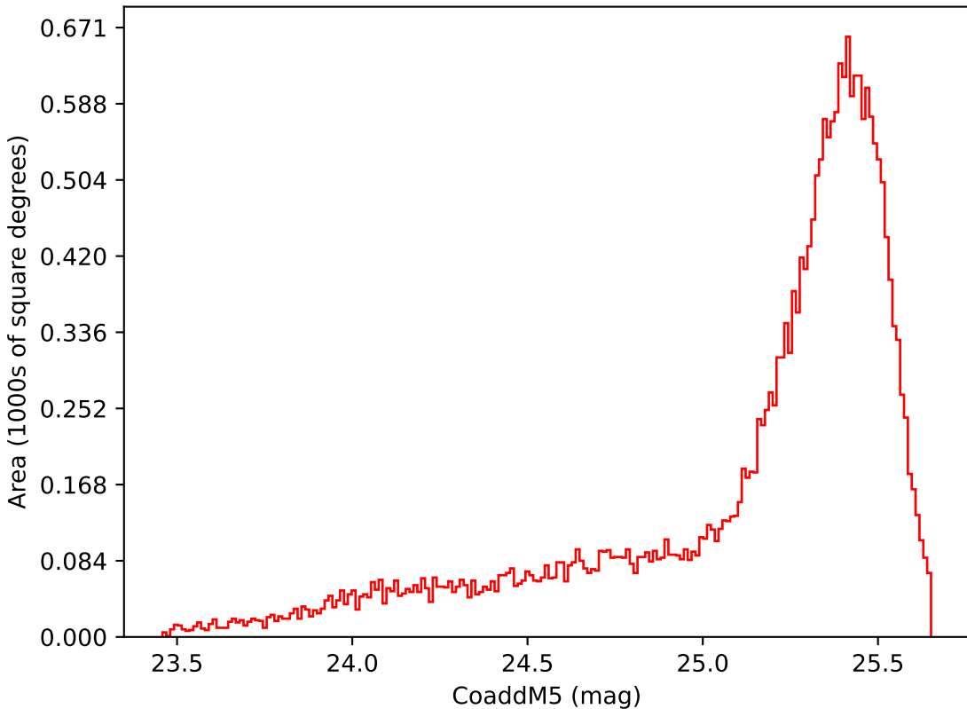
too_elab_r128_d3_gz_v3.4_10yrs Yr 1 i band: CoaddM5
