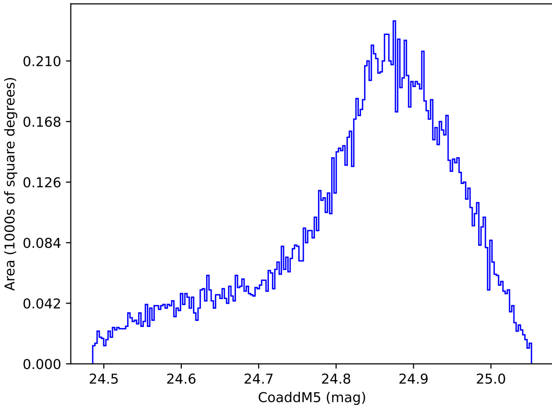
too_elab_r128_d3_gz_v3.4_10yrs WFD y band: CoaddM5
